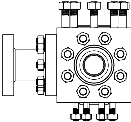
DISCHARGE MANIFOLD FACE
