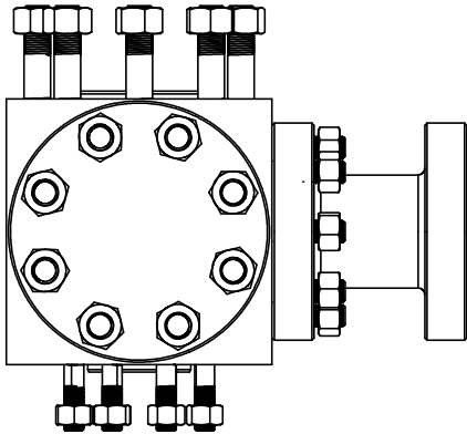
STRAINER CLEAN OUT FACE
