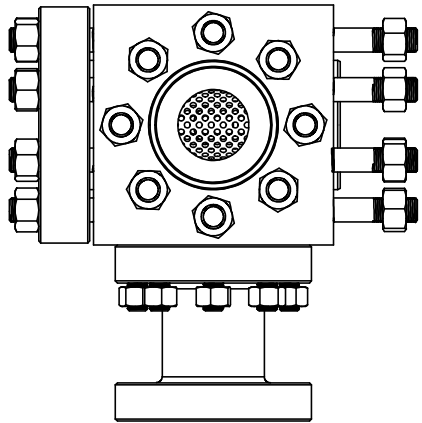
RIGHT MUD LINE FACE
