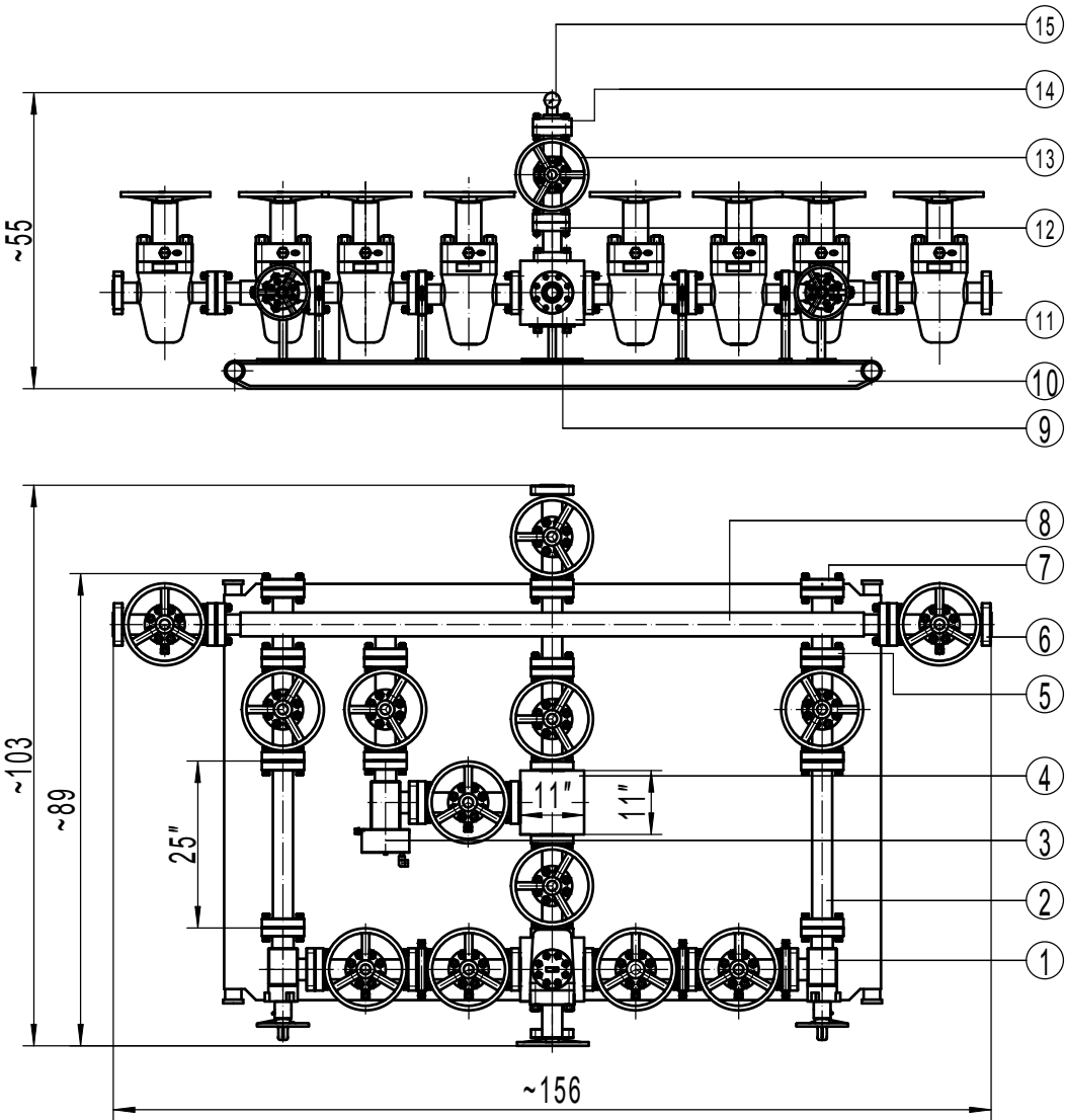
CHOKE MANIFOLD(3-1/8"5000PSI)
