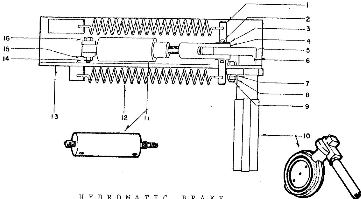
HYDROMATIC BRAKE AIR OPERATED WATER CONTROL VALVE ASS'Y 116-007-03
